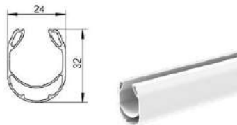
U 型下杆 U-shaped Bottom Bar T-787A-01
